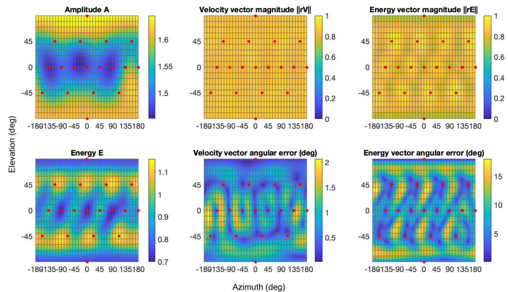
Figure 5. Distribution of the objective measures for the combination of the investigated playback system and the AllRAD. Red dots mark the loudspeaker positions. Please note that the scales for r_v angular error and energy are not equal to better visualise the differences in distributions.
