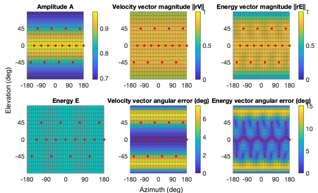
Figure 4. Distribution of the objective measures for the combination of the investigated playback system and the EPAD. Red dots mark the loudspeaker positions. Please note that the scales for r_v angular error and energy are not equal to better visualise the differences in distributions.
