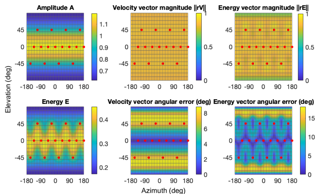
Figure 3. Distribution of the objective measures for the combination of the investigated playback system and the SAD. Red dots mark the loudspeaker positions. Please note that the scales for r_V angular error and energy are not equal to better visualise the differences in distributions.
